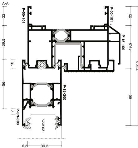
Trickle Vent Add-on to Head
