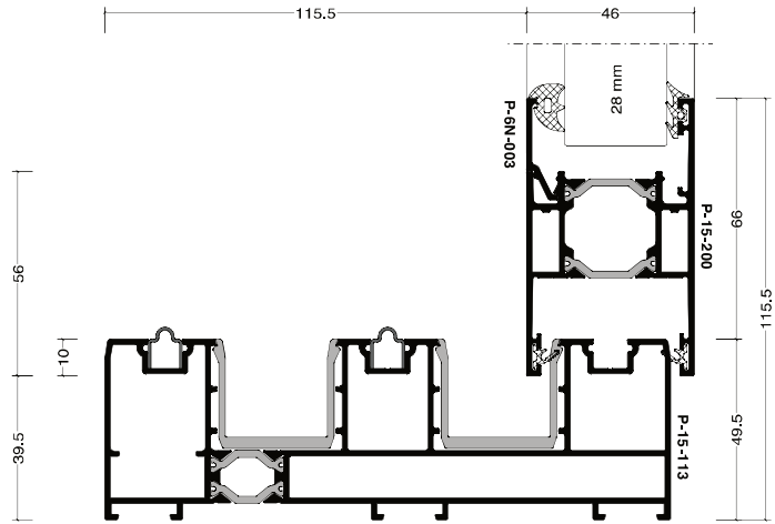
Trirail Threshold
