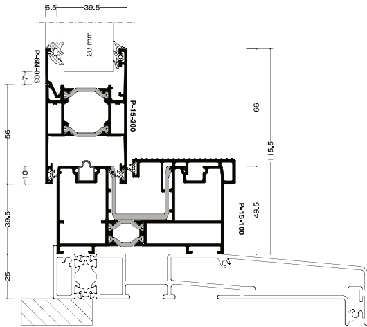
Duorail Threshold
